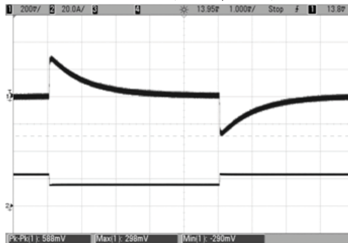
Step Load Transient Response ( V_{in} = 48V , V_{out} = \text{nom} , C_{load} = 1\mu F \parallel 10\mu F , I_{out} = 50 to 75 to 50\% of full load, T_a = +25^\circ C ) Ch1 = Vout, Ch2 = Iout.
