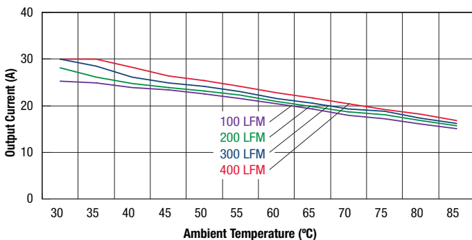
UEE-3.3/30-D48 Maximum Current Temperature Derating at Sea Level (Vin = 48V, no baseplate. Airflow direction is transverse.)
