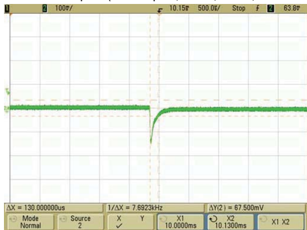
Step Load Transient Response (Slew=1A / \mu Sec., Vin=48V, Vout=nom., Iout=22.5A to 15A)
