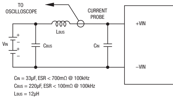
Figure 6. Measuring Input Ripple Current
