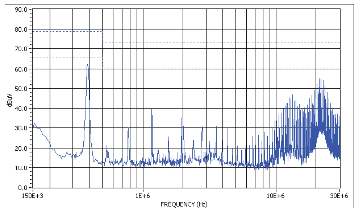
Graph 7. Conducted emissions performance, Positive Line, CISPR 22, Class A, 48 Vin, full load
