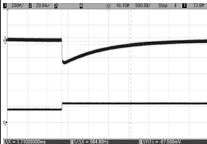
Step Load Transient Response ( V_{in} = 48V , V_{out} = \text{nom} , C_{load} = 1\mu F \parallel 10\mu F , I_{out} = 50\% to 75\% of full load, T_a = +25^\circ C ) Ch1 = Vout, Ch2 = Iout
