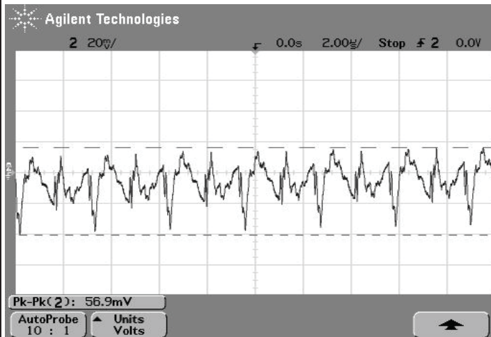
Output Ripple and noise (Vin=48V, Vout=nom., Iout=15A, Cload=0, Ta=+25° C., ScopeBW=20Mhz)
