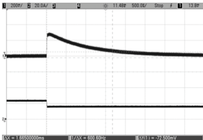
Step Load Transient Response ( V_{in} = 48V , V_{out} = \text{nom} , C_{load} = 1\mu F \parallel 10\mu F , I_{out} = 75\% to 50\% of full load, T_a = +25^\circ C ) Ch1 = Vout, Ch2 = Iout
