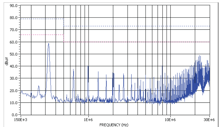
Graph 2. Conducted emissions performance, Negative Line, CISPR 22, Class A, full load
