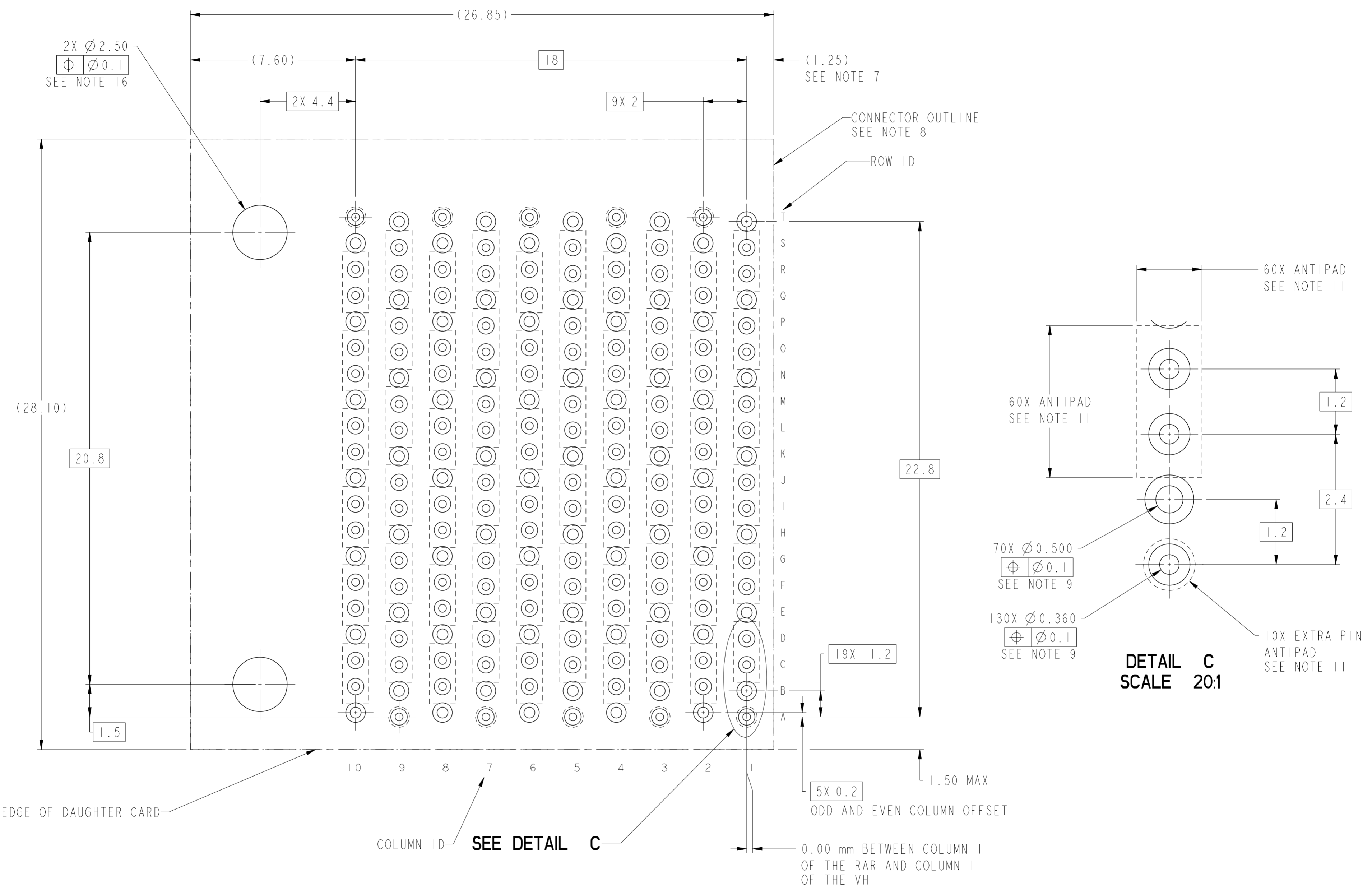
10131764-X2ALF THRU -X2JLF RECOMMENDED PCB LAYOUT COMPONENT SIDE NOTES 7, 8, 9, 11 & 16 SCALE 8:1
