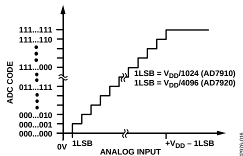
Figure 16. Transfer Characteristic
