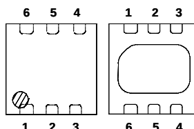
NJM2831KG1
