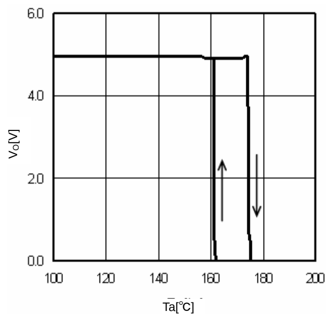
Fig.15 TSD ( I_o=0mA )
