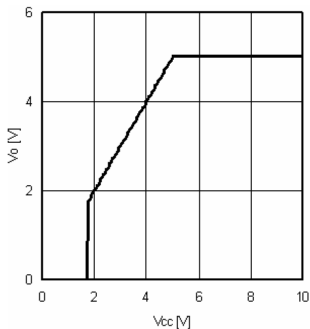
Fig.14 V_{cc}-V_o ( I_o=0mA )
