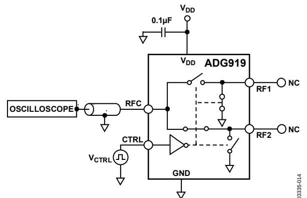
Figure 23. Video Feedthrough
