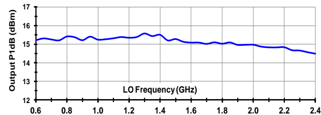
1dB Compression
