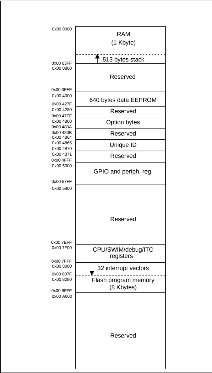
Figure 7: Memory map
