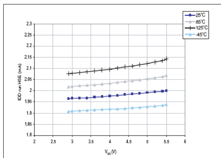
Figure 12: Typ I_{\text{DD(RUN)}} vs. V_{\text{DD}} HSE user external clock, f_{\text{CPU}} = 16 \text{ MHz}
