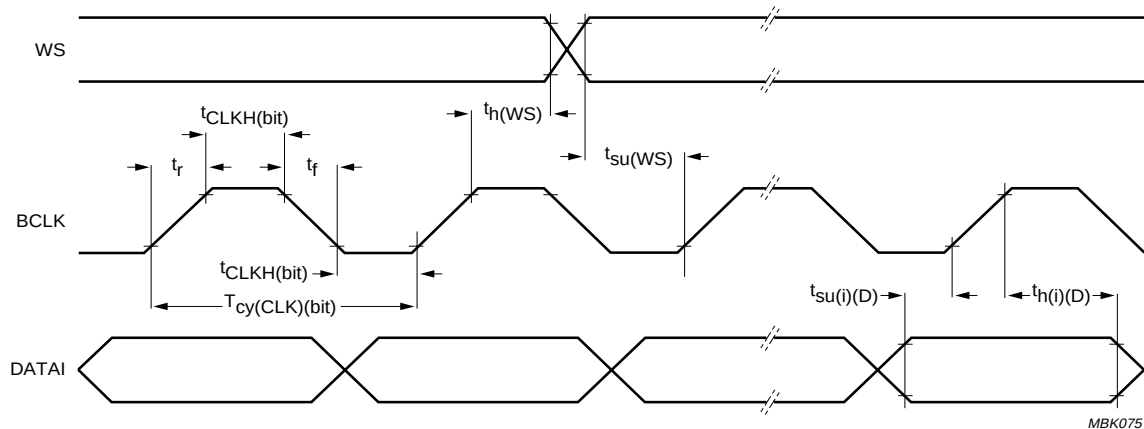
Fig.7 Serial interface timing.
