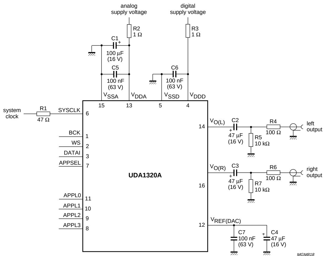
Fig.8 Application schematic.
