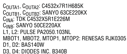
Figure 14. High Efficiency 2-Phase 24V Boost Converter with Inductor DCR Current Sensing
