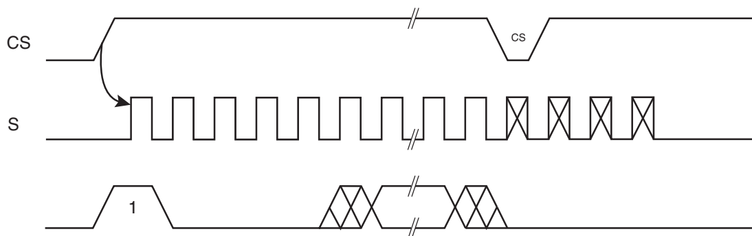
Figure 3-4. EWDS Timing
