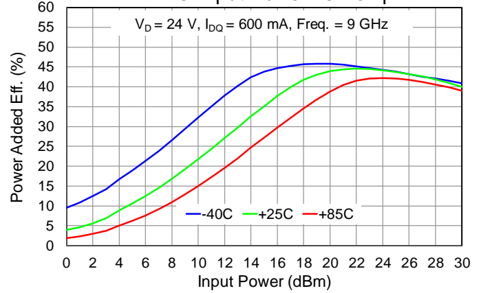
PAE vs. Input Power vs. Temp.
