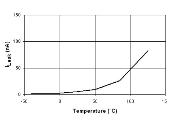
Figure 24. Switch leakage vs. temperature (STMP2141/2151)
