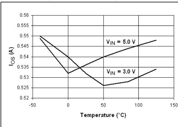
Figure 23. I_{OS} vs. temperature (STMP2141/2151)
