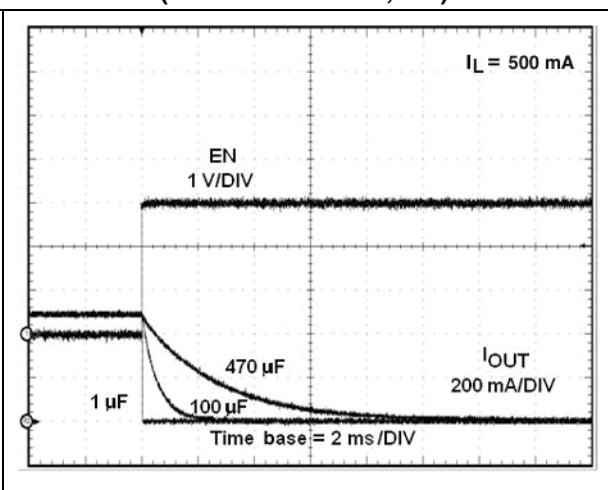
Figure 10. Current output turn-off delay time (STMPS2141/2151, 3 V)
