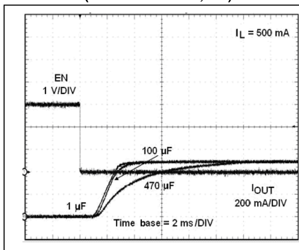
Figure 9. Current output turn-on delay time (STMPS2141/2151, 3 V)
