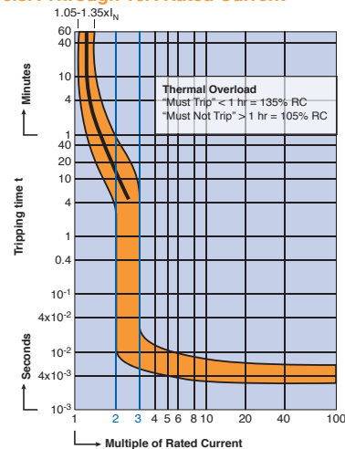
V-EA-Z Trip 0.3A Through 10A Rated Current
