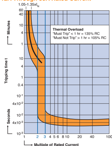
V-EA-Z Trip 12A Through 50A Rated Current
