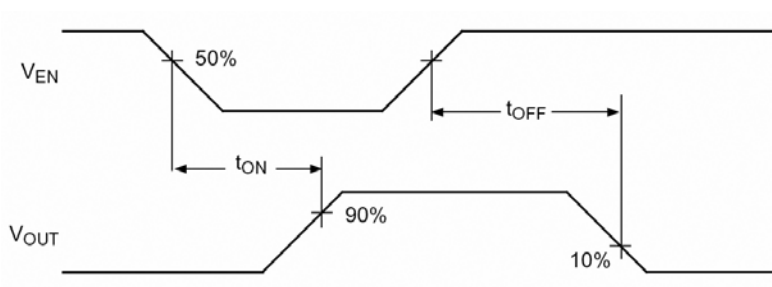
Figure 1b. MIC2544A-2/MIC2548A-2
