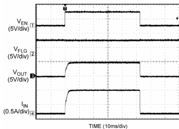
Enable Turn-On/Turn-Off
