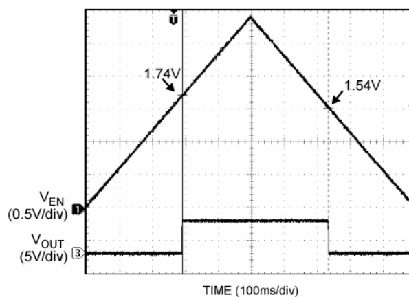
Enable Thresholds
