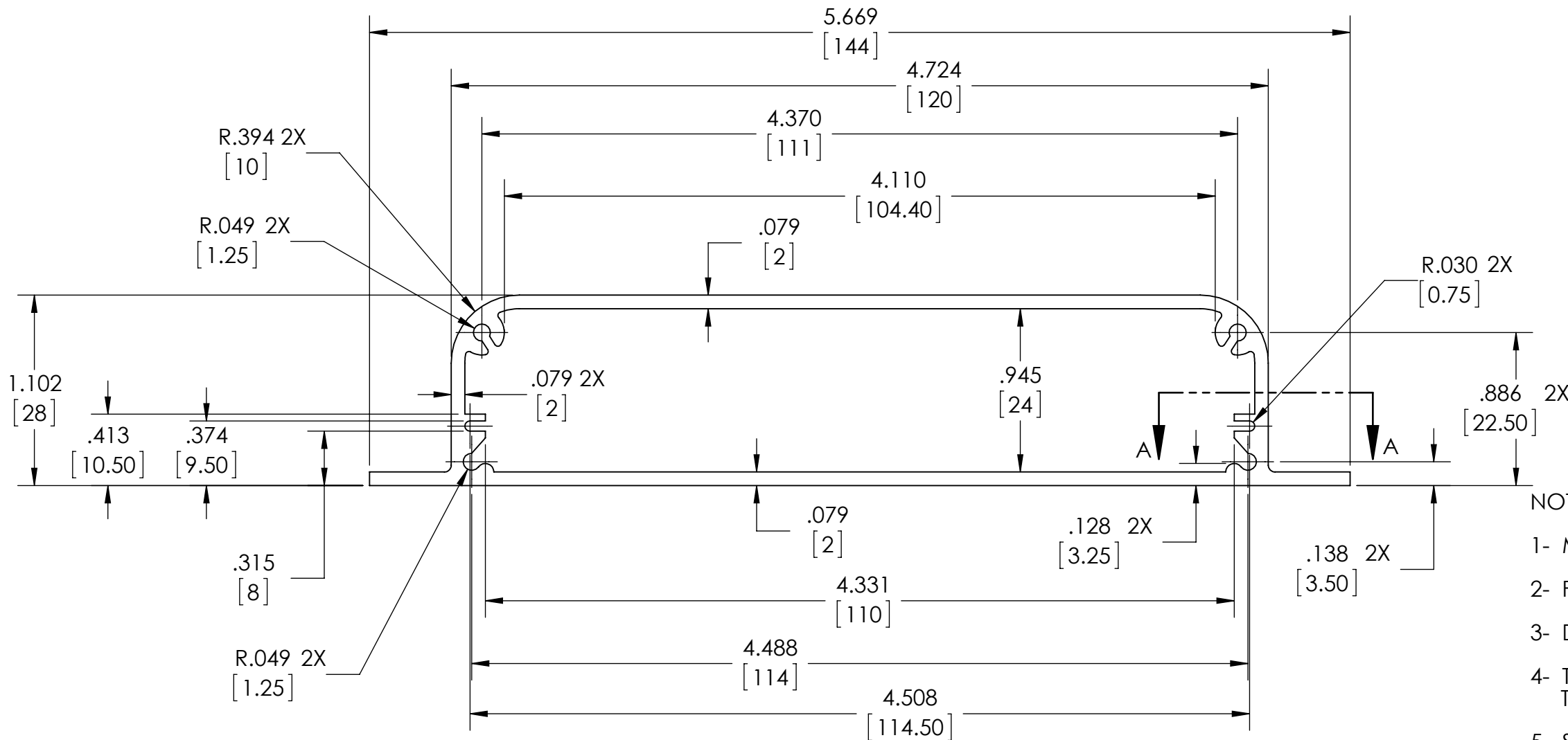
EXTRUSION PROFILE
