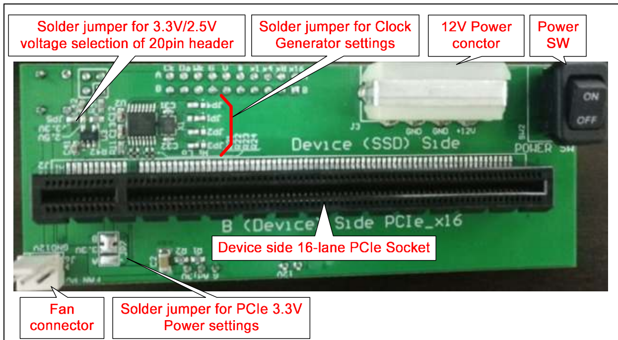
Figure-2: Board device (B) side
