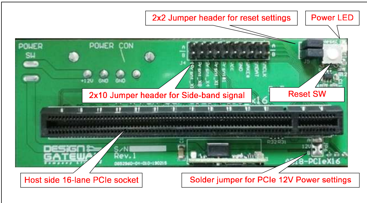
Figure-1: Board host (A) side
