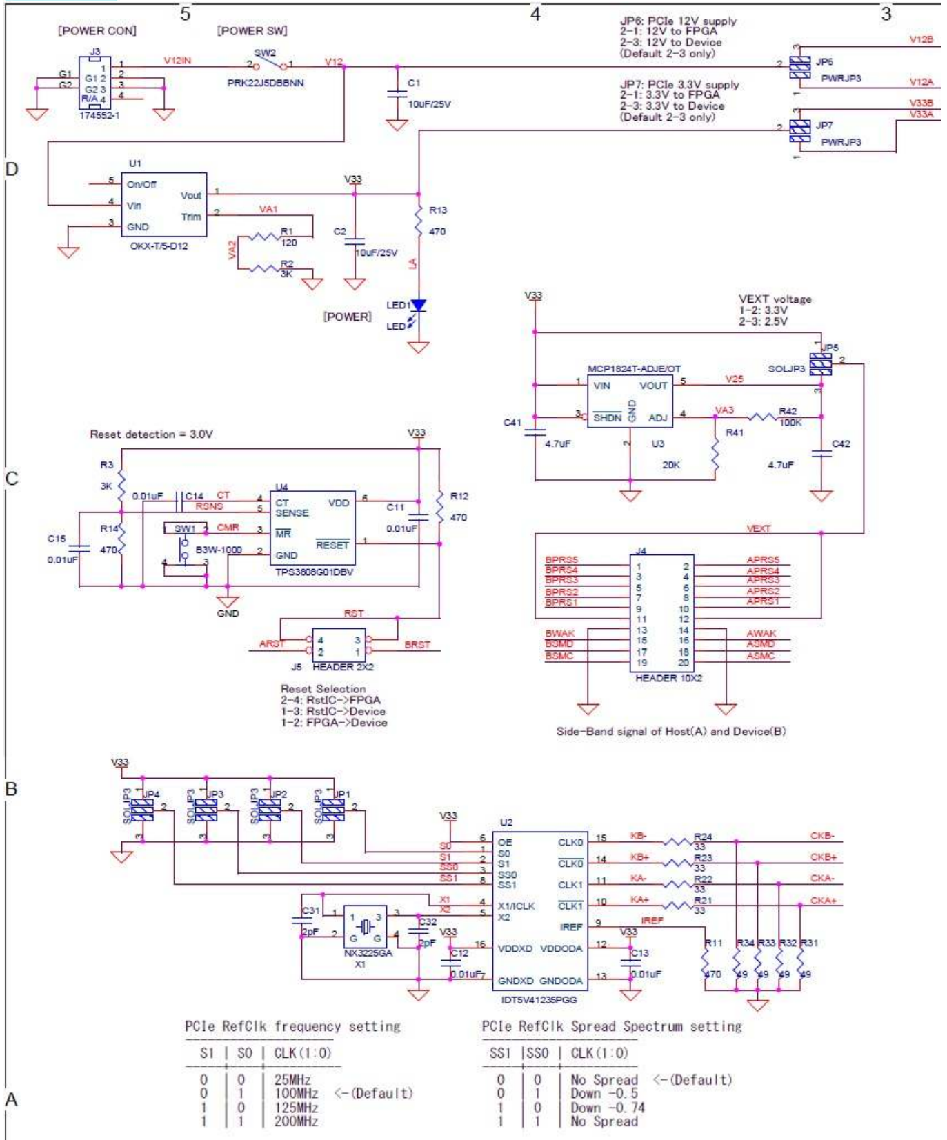
Figure-10: Adapter board schematic (1 of 2)
