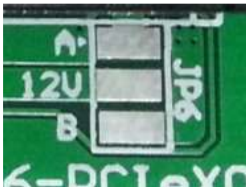
Figure8:: JP6 soldering can select 12V PCIe power supply to host/device side
