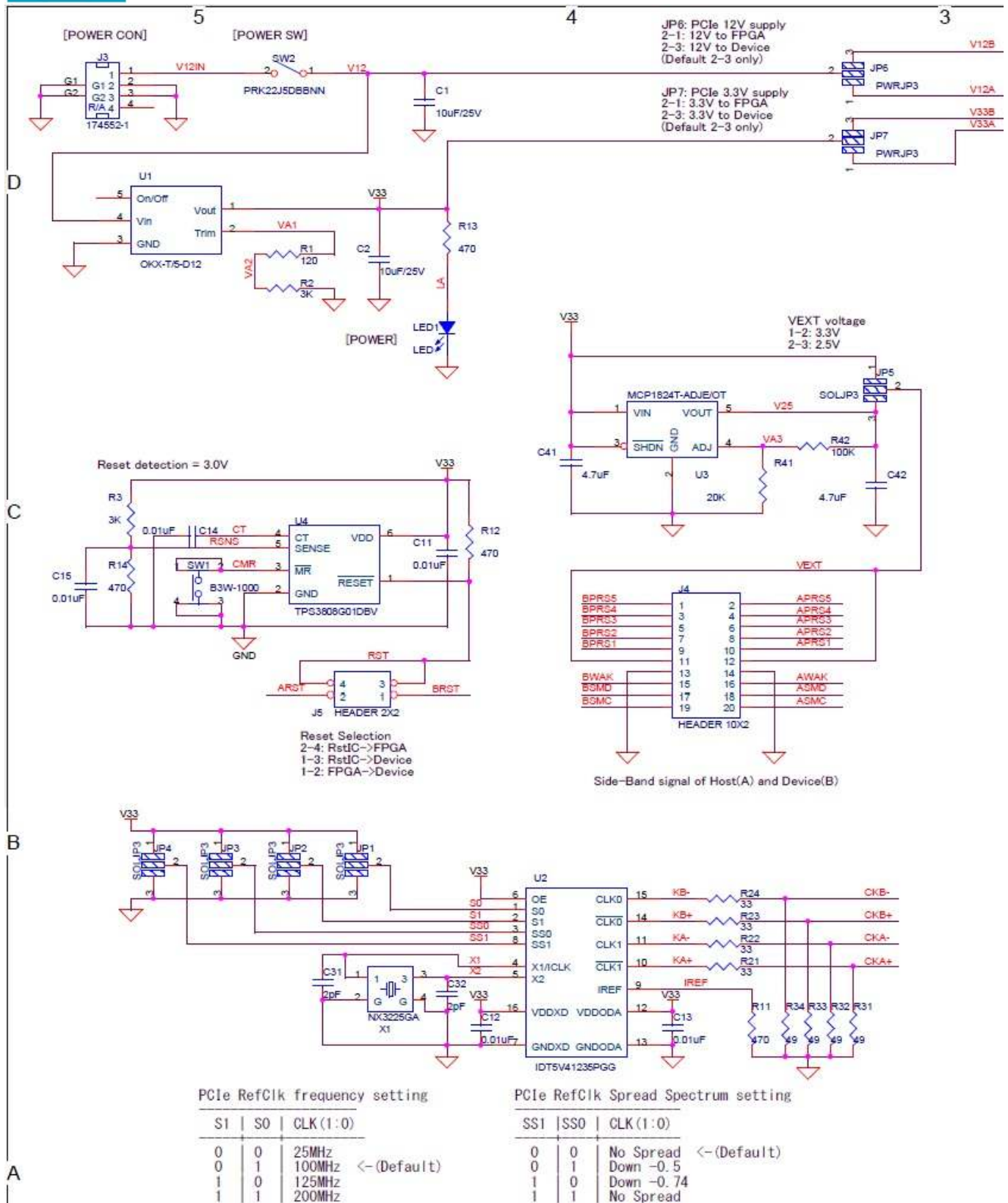
Figure-10: Adapter board schematic (1 of 2)
