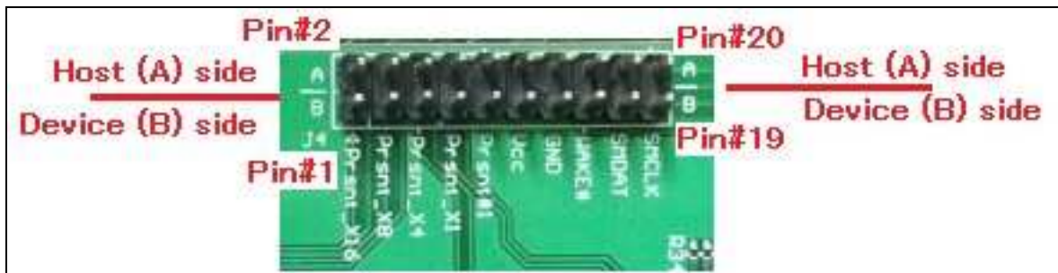
Figure-3: J4 pin header for PCIe side-band signal
