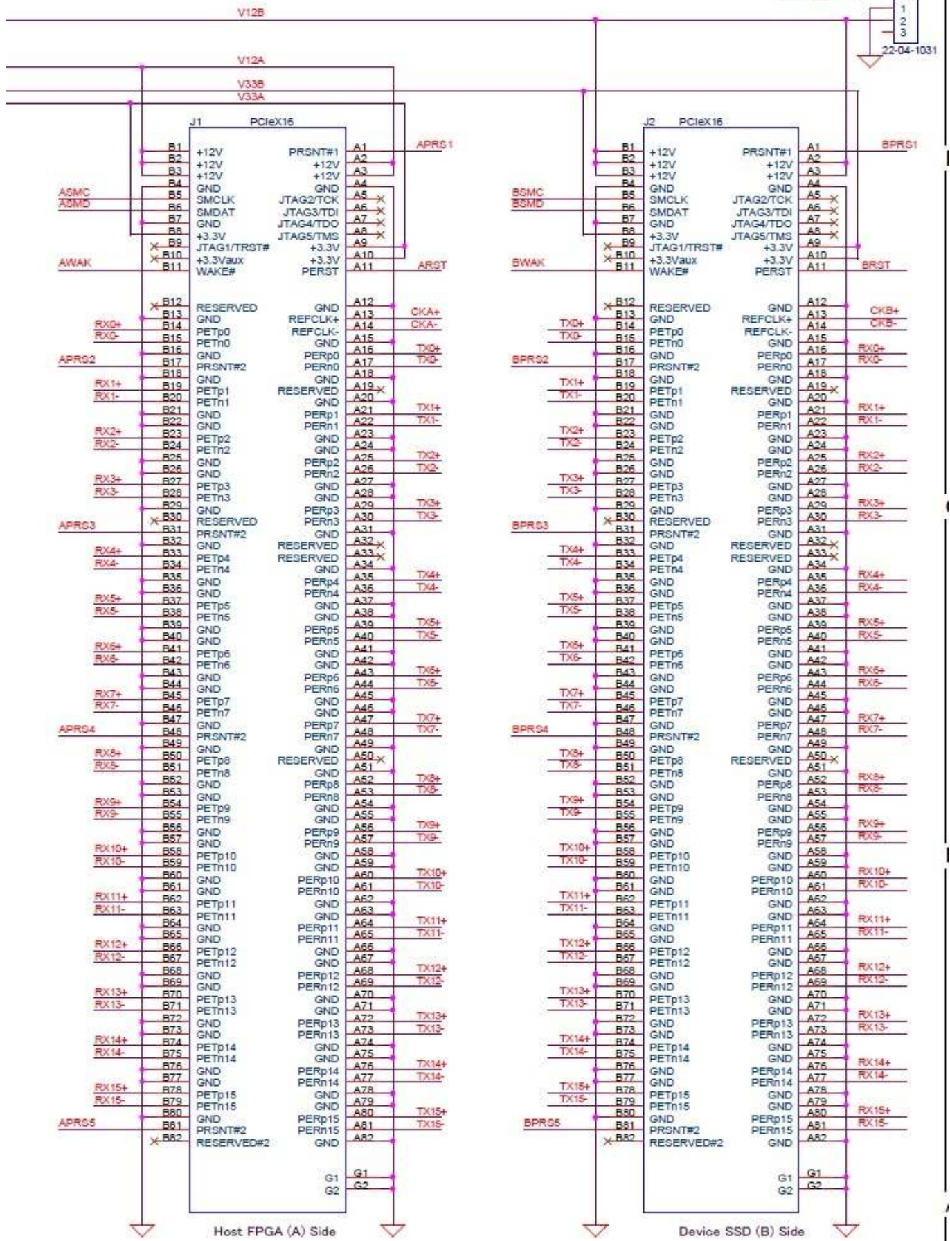
Figure-11: Adapter board schematic (2 of 2)
