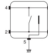
Terminal Arrangement /Internal Connections (Top View)
