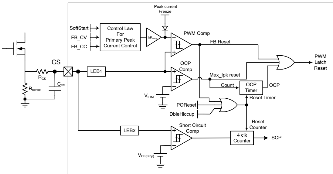
Figure 53. Current Setpoint
