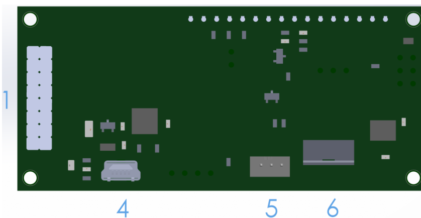
Figure 3: OK162-12-USB Header Locations
