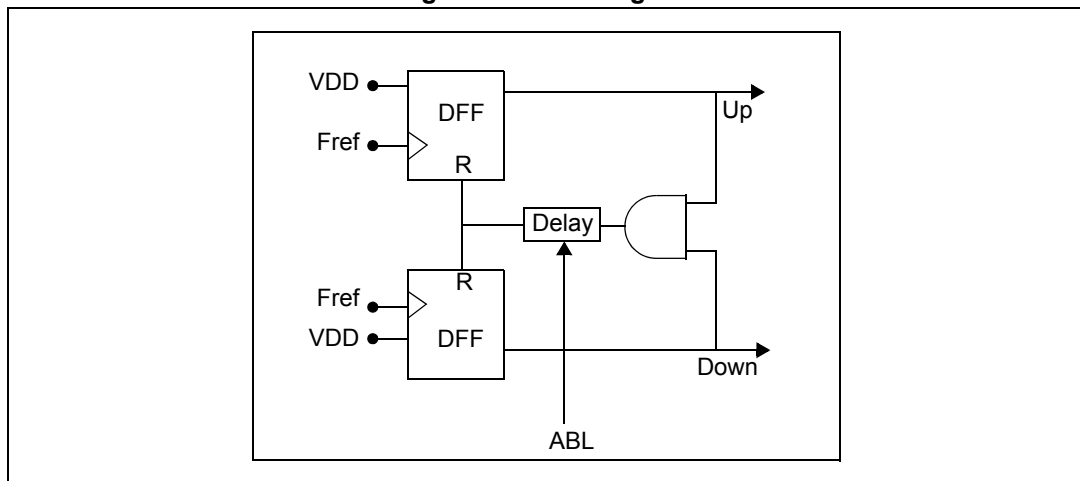
Figure 30. PFD diagram
