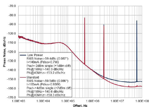
Figure 11. Phase noise and fractional spurs at 2118.24 MHz at 5.0 V supply ( F_{\text{PFD}} = 61.44 \text{ MHz} )
