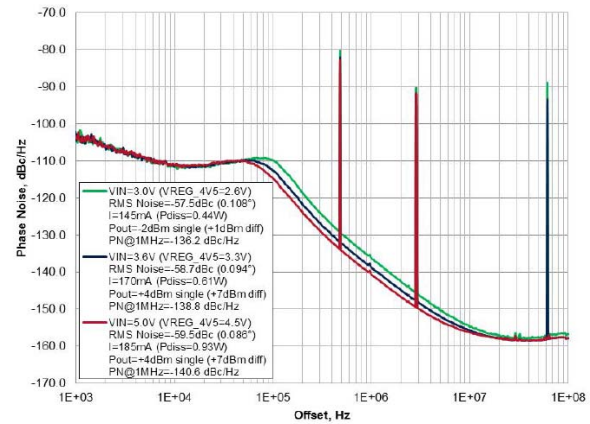
Figure 10. Phase noise and fractional spurs at 2118.24 MHz vs. supply ( F_{\text{PFD}} = 61.44 \text{ MHz} )
