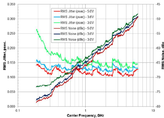
Figure 7. Single sideband integrated phase noise vs. frequency and supply ( F_{\text{PFD}} = 50 \text{ MHz} )
