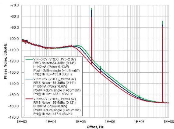
Figure 9. Phase noise and fractional spurs at 2646.96 MHz vs. supply ( F_{\text{PFD}} = 61.44 \text{ MHz} )
