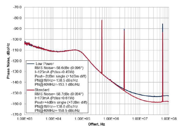
Figure 12. Phase noise and fractional spurs at 2118.24 MHz at 3.6 V supply ( F_{\text{PFD}} = 61.44 \text{ MHz} )
