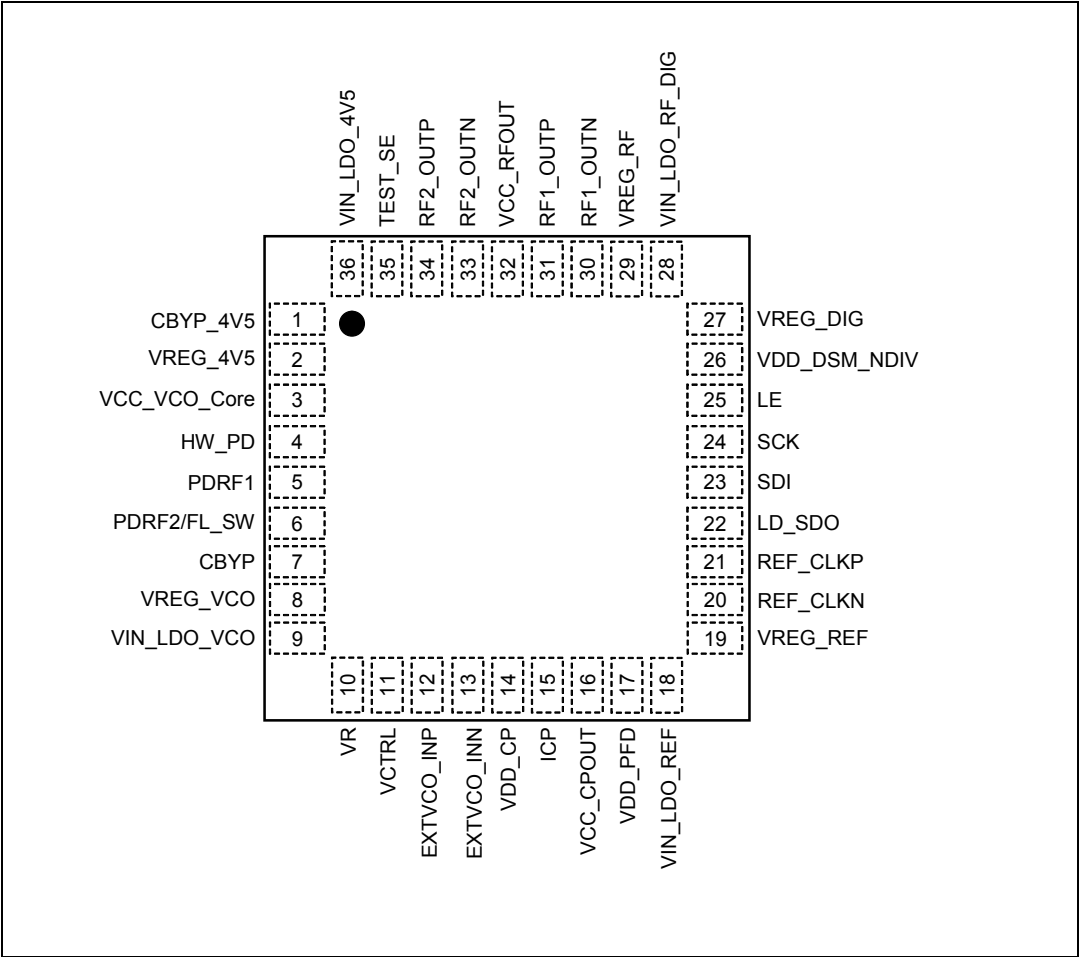
Figure 2. Top view
