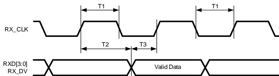
Figure 11. 10Mb/s MII Receive Timing
