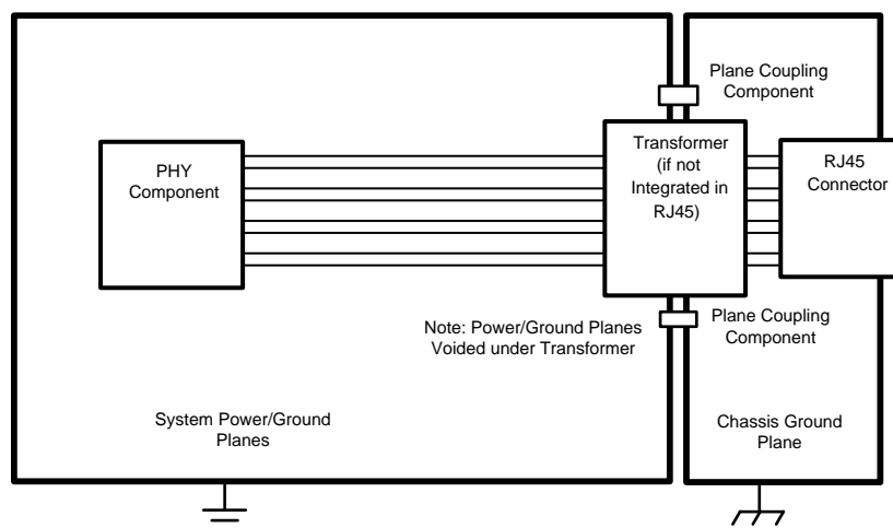
Figure 36. Layout Example
