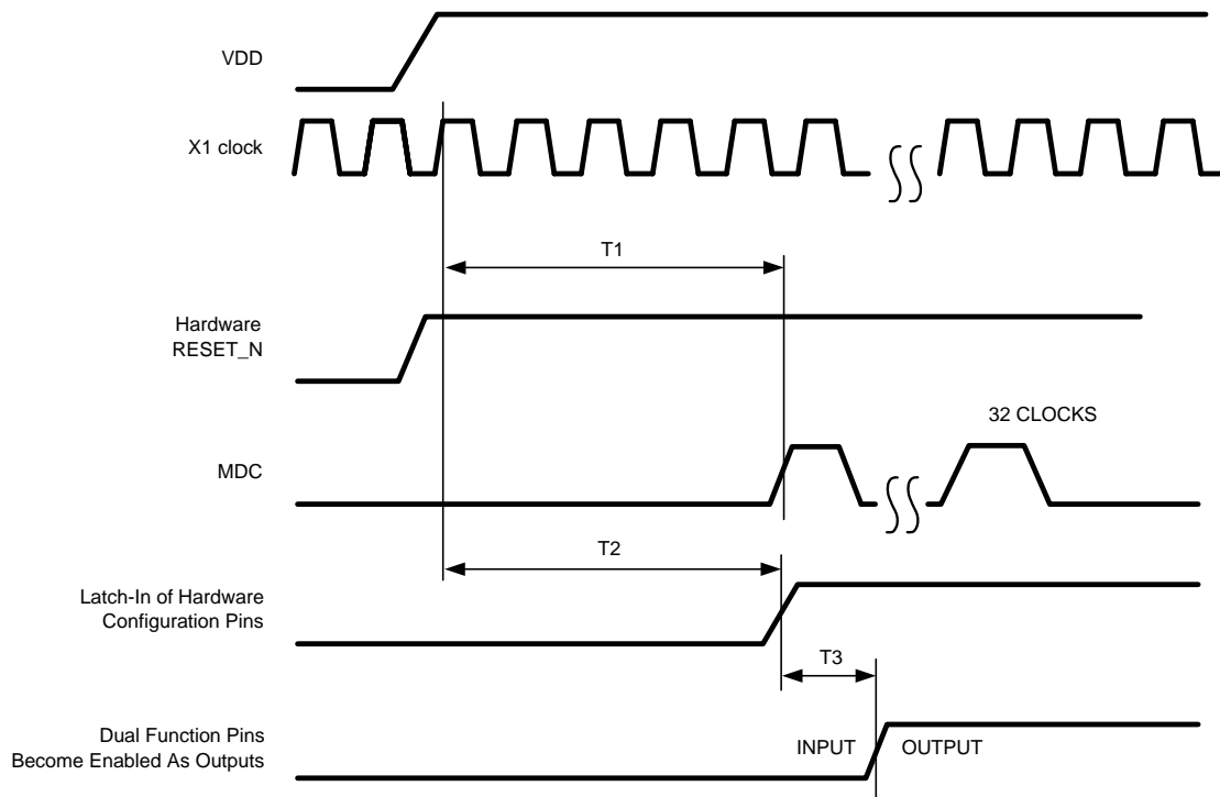
Figure 1. Powerup Timing
