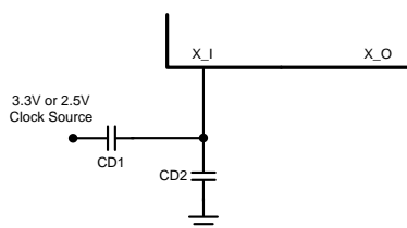
Figure 28. Clock Divider
