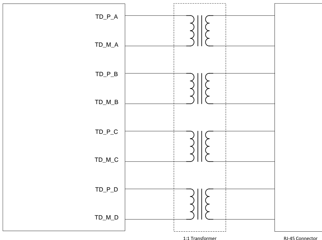
Figure 27. Magnetics Connections
