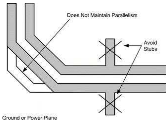
Figure 32. Avoiding Stubs in a Differential Signal Pair
