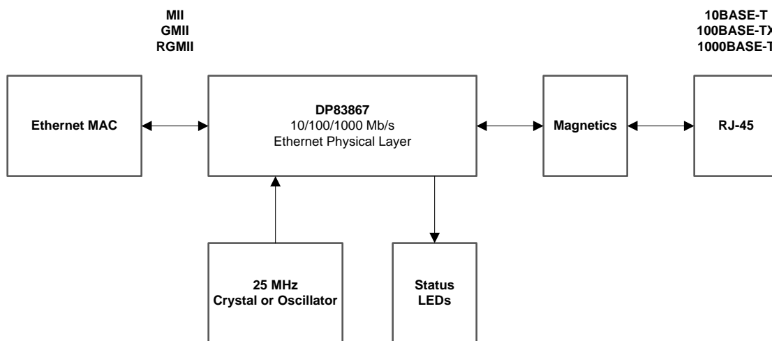
Figure 26. Typical DP83867 Application
