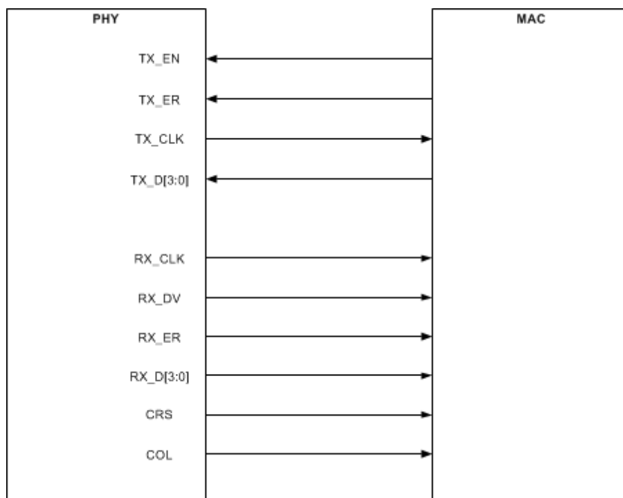
Figure 18. MII Connections
