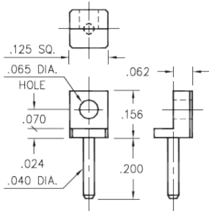
3621-0-32-XX-00-00-08-0 Board edge rivet mount
