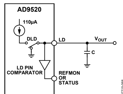
Figure 44. Current Source Digital Lock Detect
