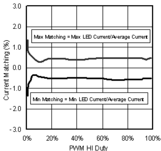
Figure 20. LED current matching - PWMPOW-HI Duty PWM = 200Hz
