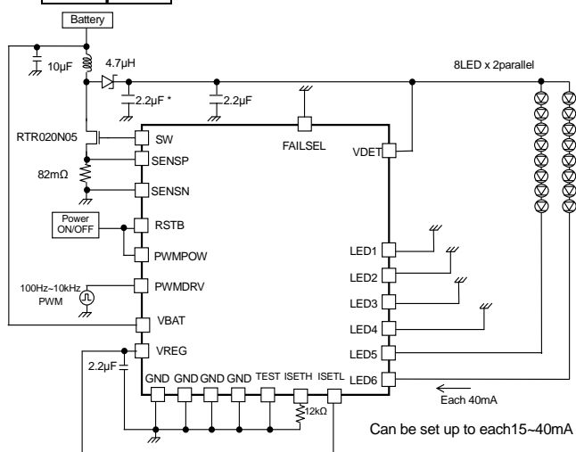
Figure 56. 8 seriesx2 parallel, LED current 40mA setting Current driver PWM application
