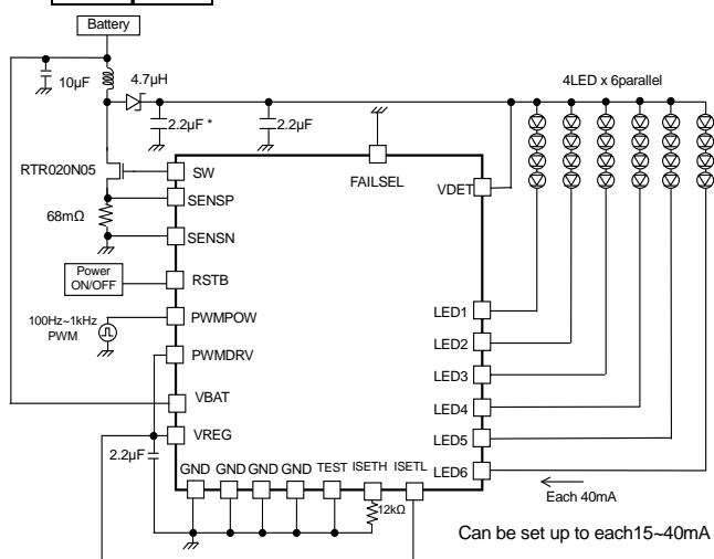
Figure 54. 4 seriesx6 parallel, LED current 40mA setting Power control PWM application
