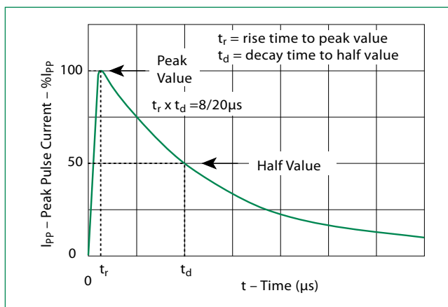
Figure 2 - Pulse Waveform
