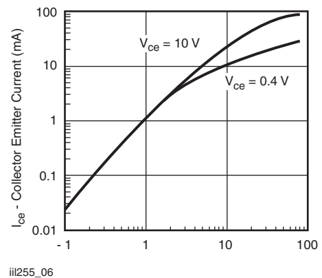
Fig. 6 - Non-Saturated and Saturated Collector Emitter Current vs. LED Current
