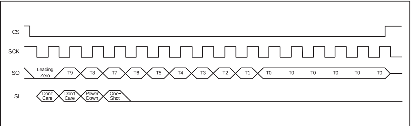
Figure 4. One-Shot Command
