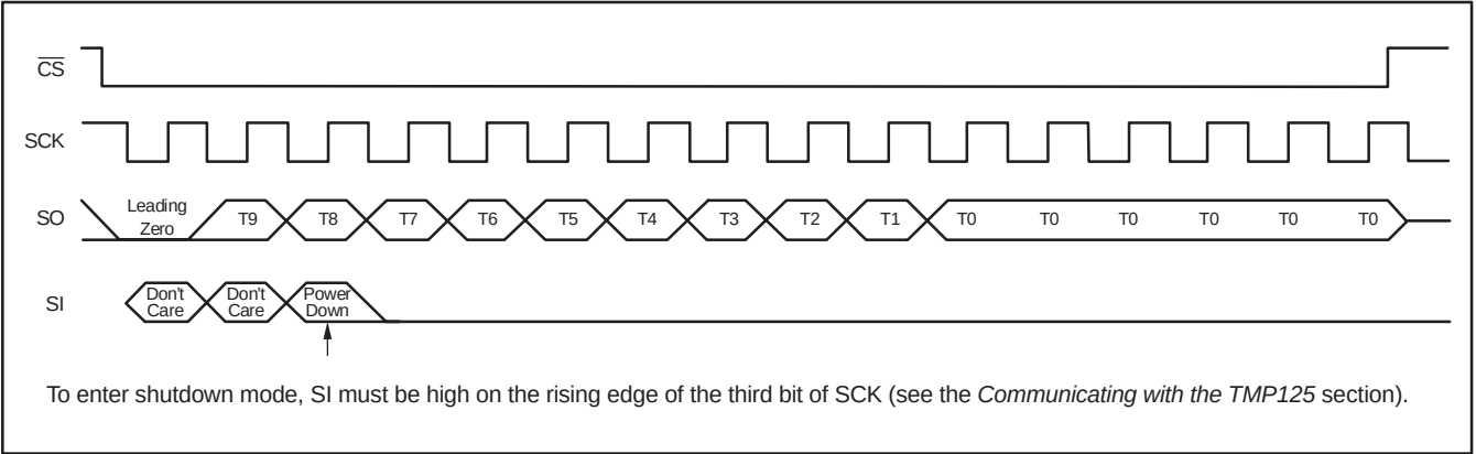
Figure 3. Data READ
