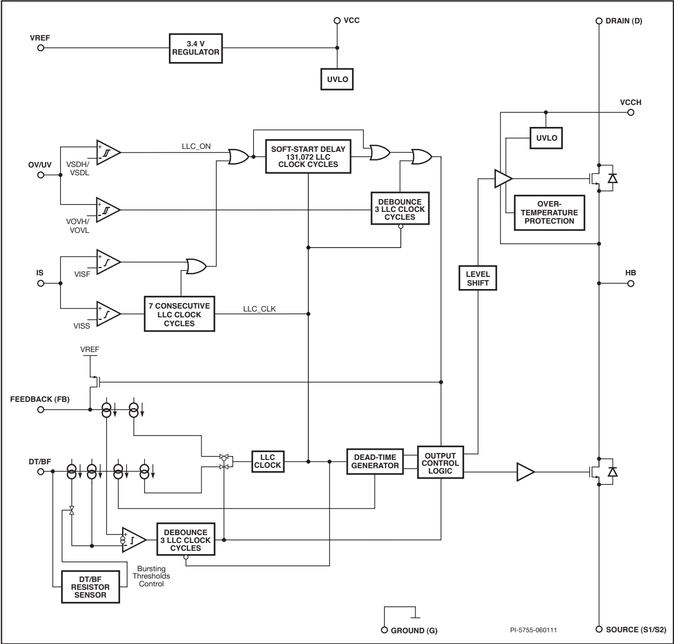
Figure 2. Block Diagram.
