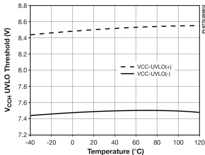
Figure 43. Typical V_{CH UVLO} vs. Temperature.
