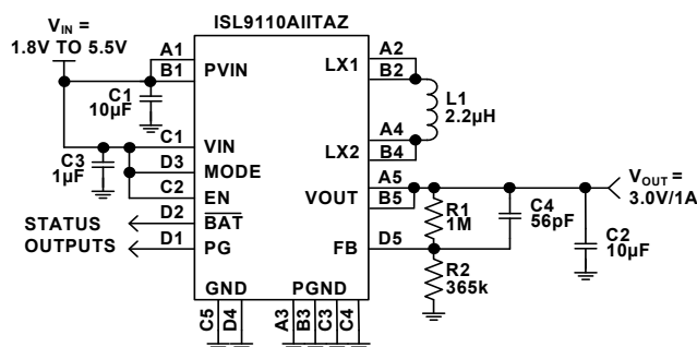
FIGURE 28. TYPICAL ISL9110AITAZ APPLICATION
