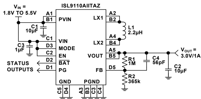
FIGURE 28. TYPICAL ISL9110AIIITAZ APPLICATION
