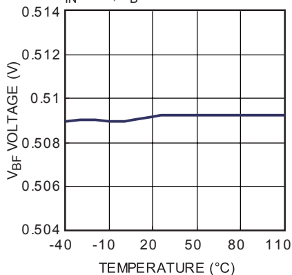
V_{BF} vs. Temperature V_{IN}=1.5V , V_B=3.6V
