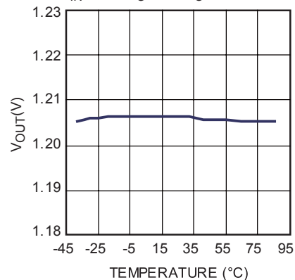
V_{OUT} vs. Temperature V_{IN}=1.5V , V_O=1.5V , I_O=1mA
