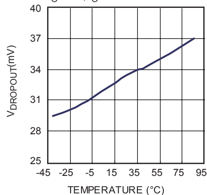
V_{DROPOUT} vs. Temperature V_O=1.2V , I_O=1A
