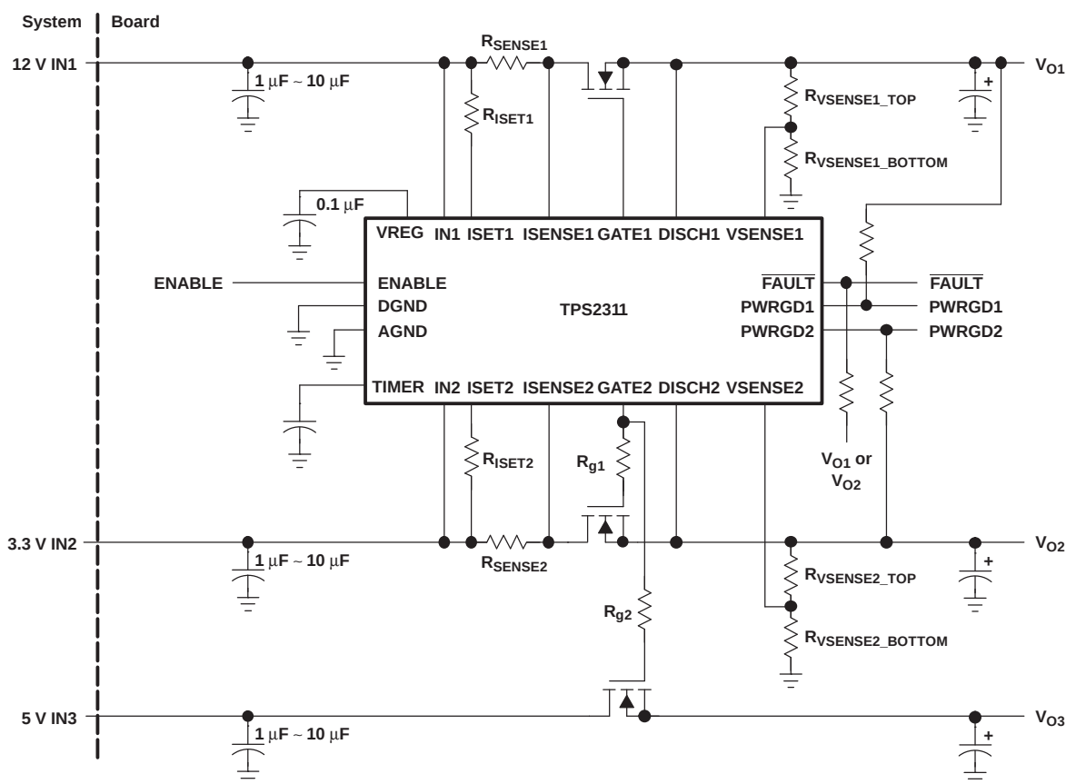
Figure 28. Three-Channel Application
