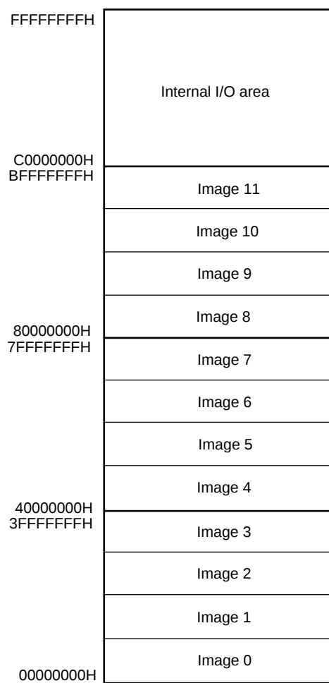
Figure 2-3. Image Space Used When Chip Select Function is Used
