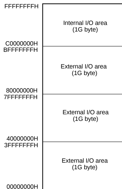
Figure 2-2. I/O Map
