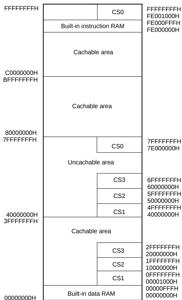
Figure 2-1. Memory Map
