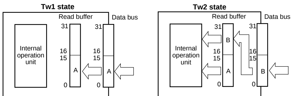
Figure 4-3. Read Cycle
