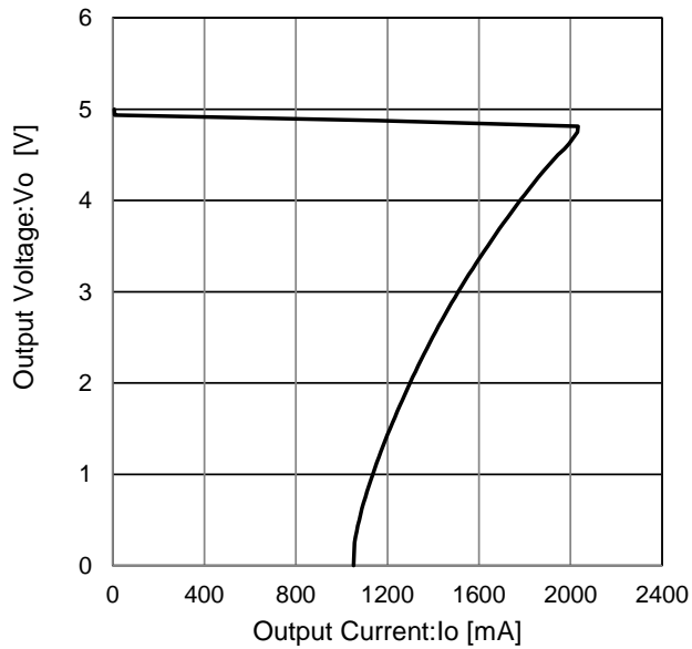
Figure 8. Load Regulation
