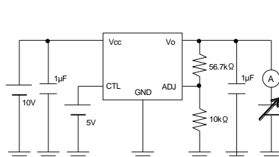
Measurement Circuit of Figure 8
