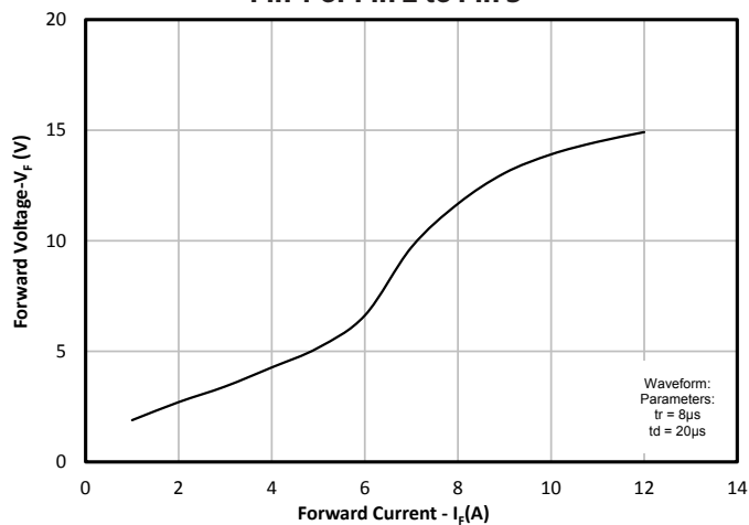
Forward Voltage vs. Forward Current ( t_p=8/20\mu s ) Pin 1 or Pin 2 to Pin 3
