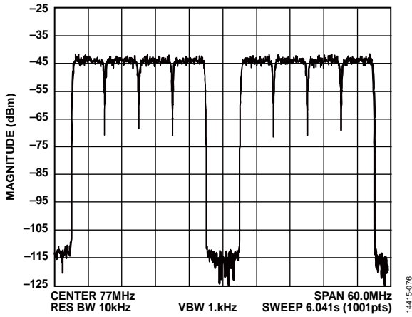
Figure 83. Gap Channel ACLR at 77 MHz
