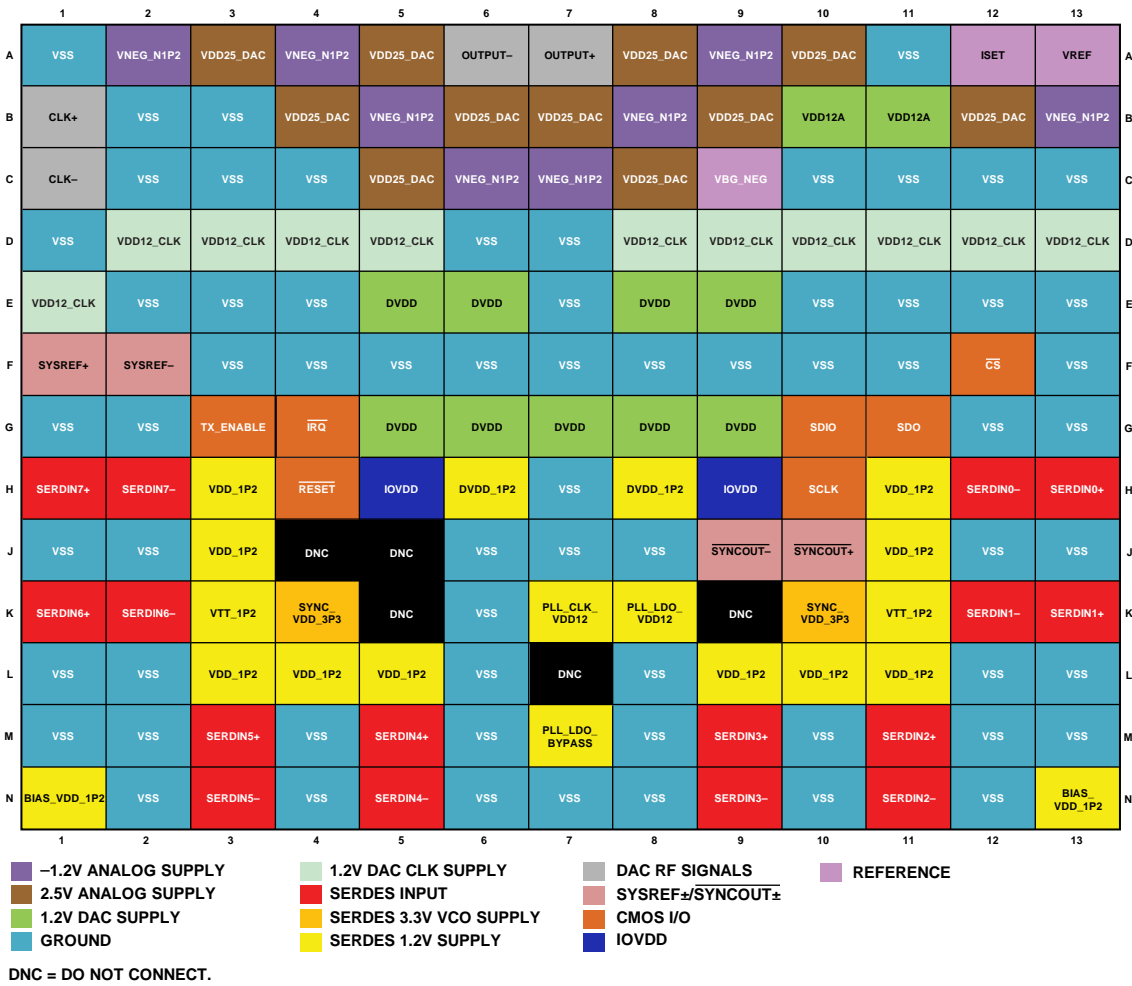
Figure 4. 169-Ball CSP_BGA Pin Configuration
