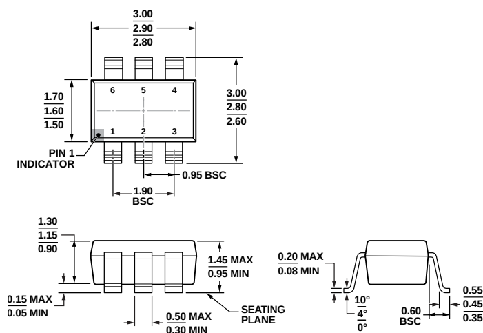
Figure 60. 6-Lead Small Outline Transistor Package [SOT-23] (RJ-6) Dimensions shown in millimeters
