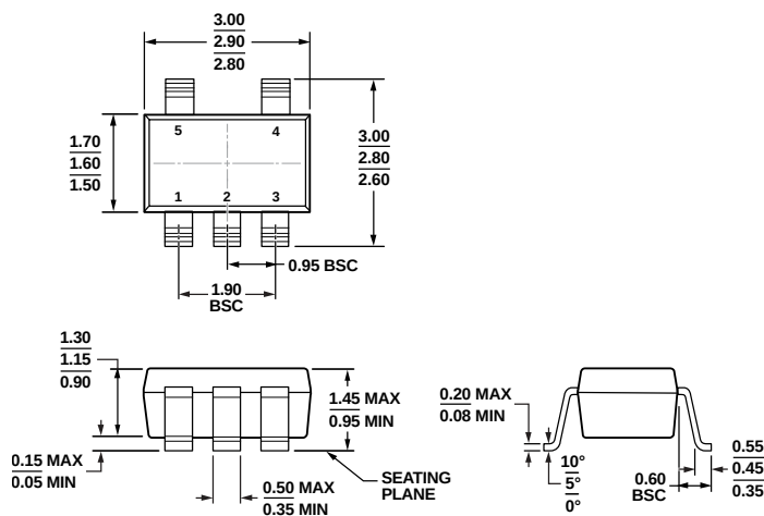
Figure 58. 5-Lead Small Outline Transistor Package [SOT-23] (RJ-5) Dimensions shown in millimeters
