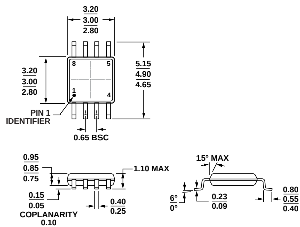
Figure 61. 8-Lead Mini Small Outline Package [MSOP] (RM-8) Dimensions shown in millimeters
