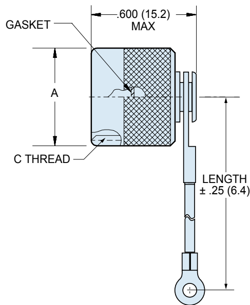
667-185 Receptacle Cover
