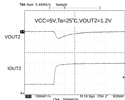
Fig.22 V_{OUT2} Transient Response ( I_o 0.5A \rightarrow 1.5A / usec)
