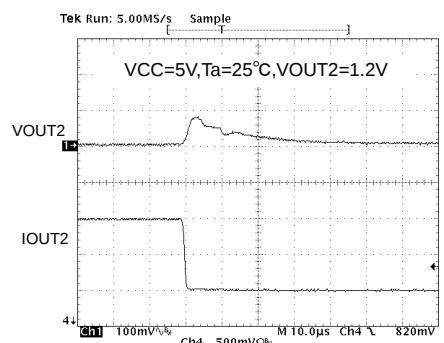
Fig.23 V_{OUT2} Transient Response ( I_o 1.5A \rightarrow 0.5A / usec)
