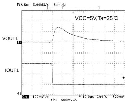
Fig.21 V_{OUT1} Transient Response ( I_o 1.5A \rightarrow 0.5A / usec)
