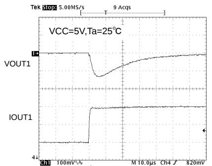
Fig.20 V_{OUT1} Transient Response ( I_o 0.5A \rightarrow 1.5A / usec)
