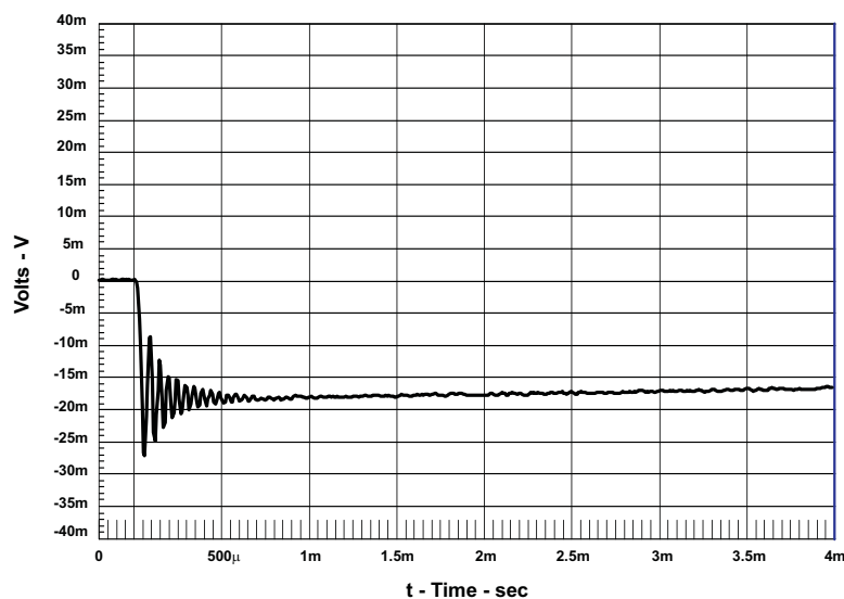
Figure 20. Pop/Click (PBTL)
