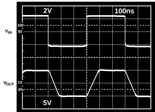
Figure 41. Output Waveform of an AD811 Driving a 500 pF Load. Gain = +2, R_{FB} = 649 \Omega , R_S = 15 \Omega , R_L = 10 \text{ k}\Omega
