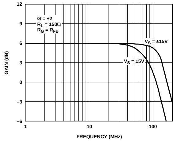
Figure 6. Frequency Response
