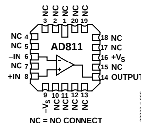
Figure 3. 20-Terminal LCC (E-20A)
