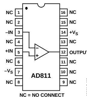
Figure 2. 16-Lead SOIC (R-16)
