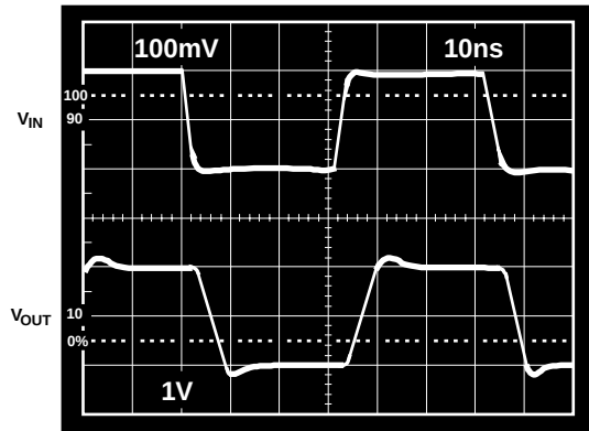
Figure 27. Small Signal Pulse Response, Gain = +1
